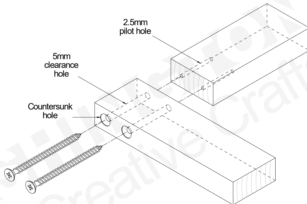
Exploded Joint
