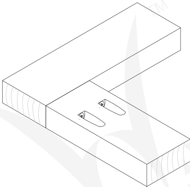
Assembled Joint
