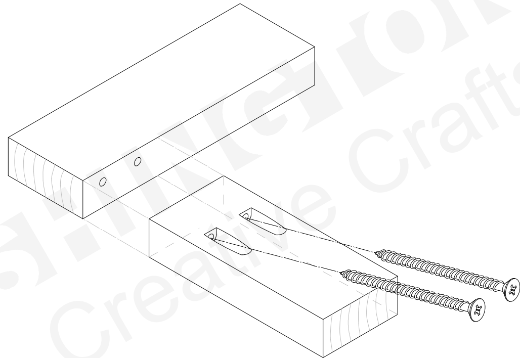
Exploded Joint
