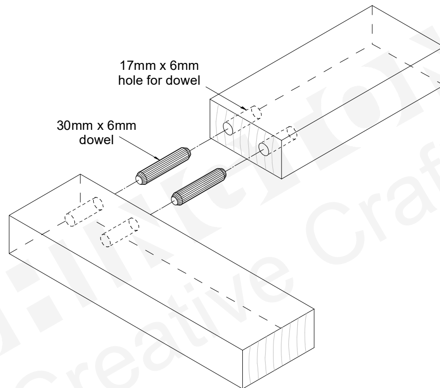
Exploded Joint
